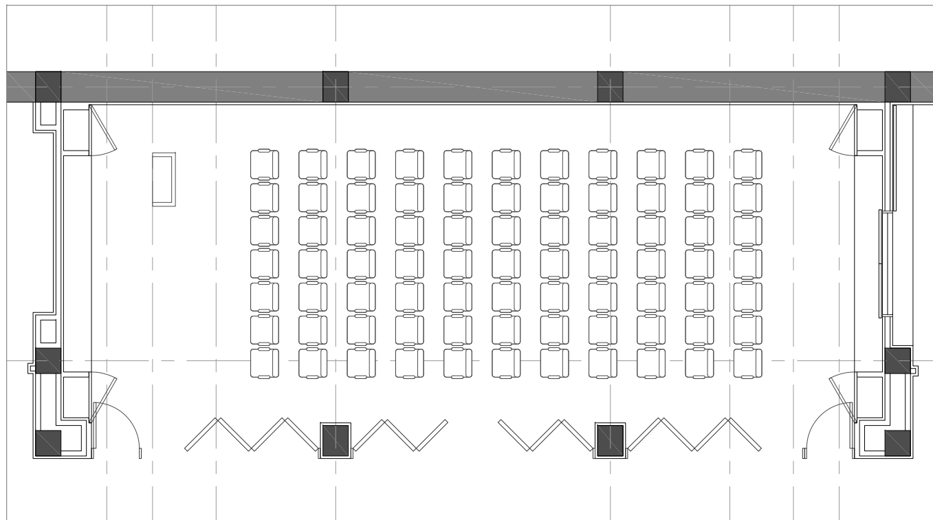
3 THEATER SEATING - SCHEME A ( 77 P )
