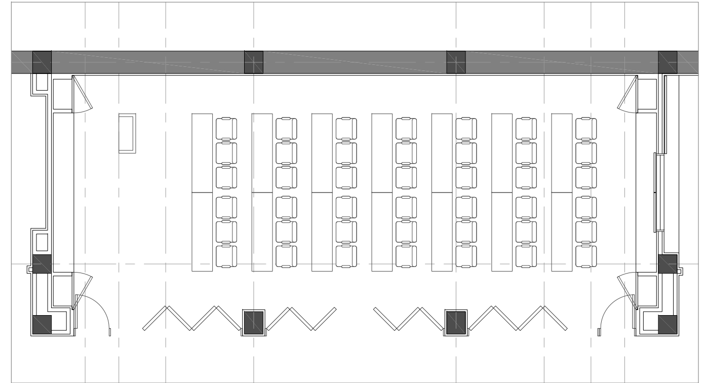
2 CLASSROOM SEATING - SCHEME A ( 42 P )
