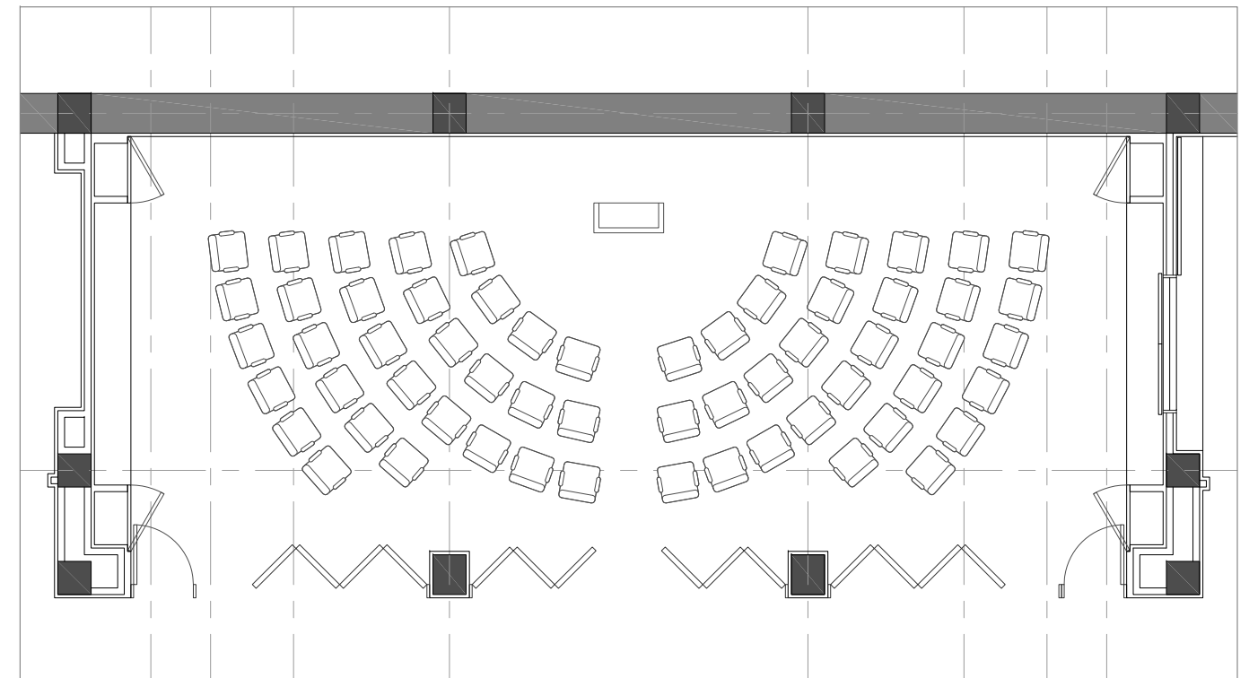
4 THEATER SEATING - SCHEME B ( 60 P )
